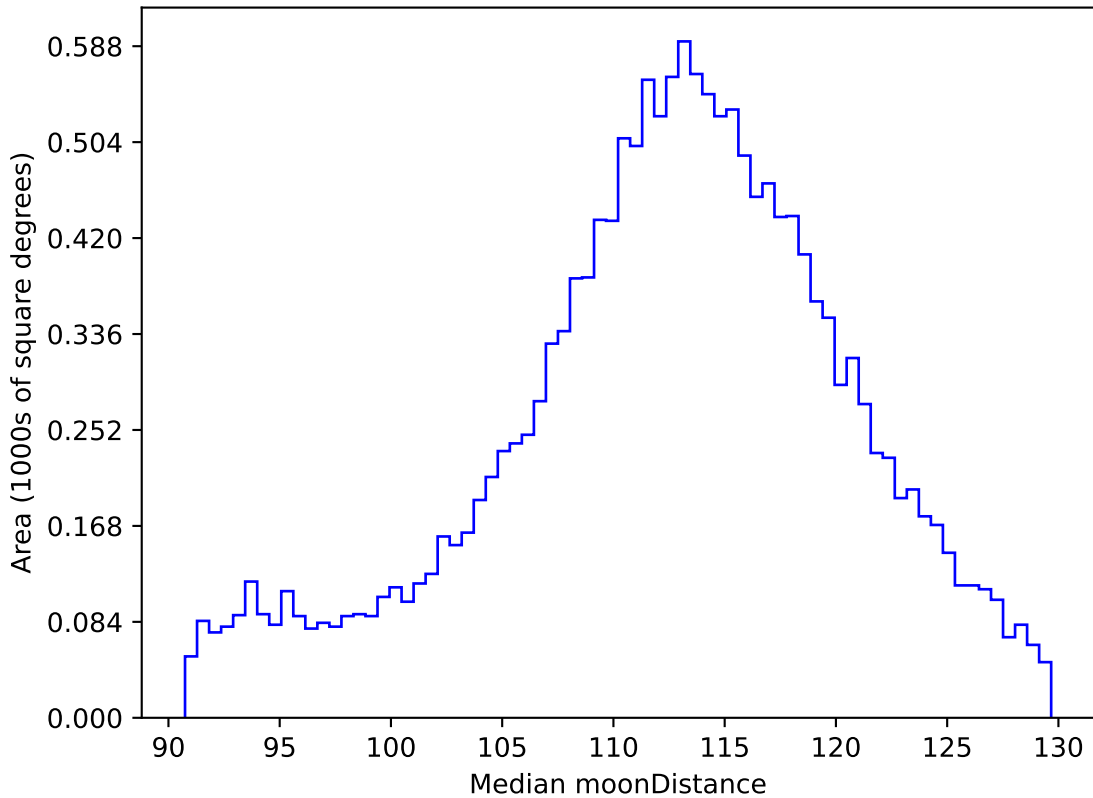
too_elab_r256_d3_griz_v3.4_10yrs WFD r band: Median moonDistance
