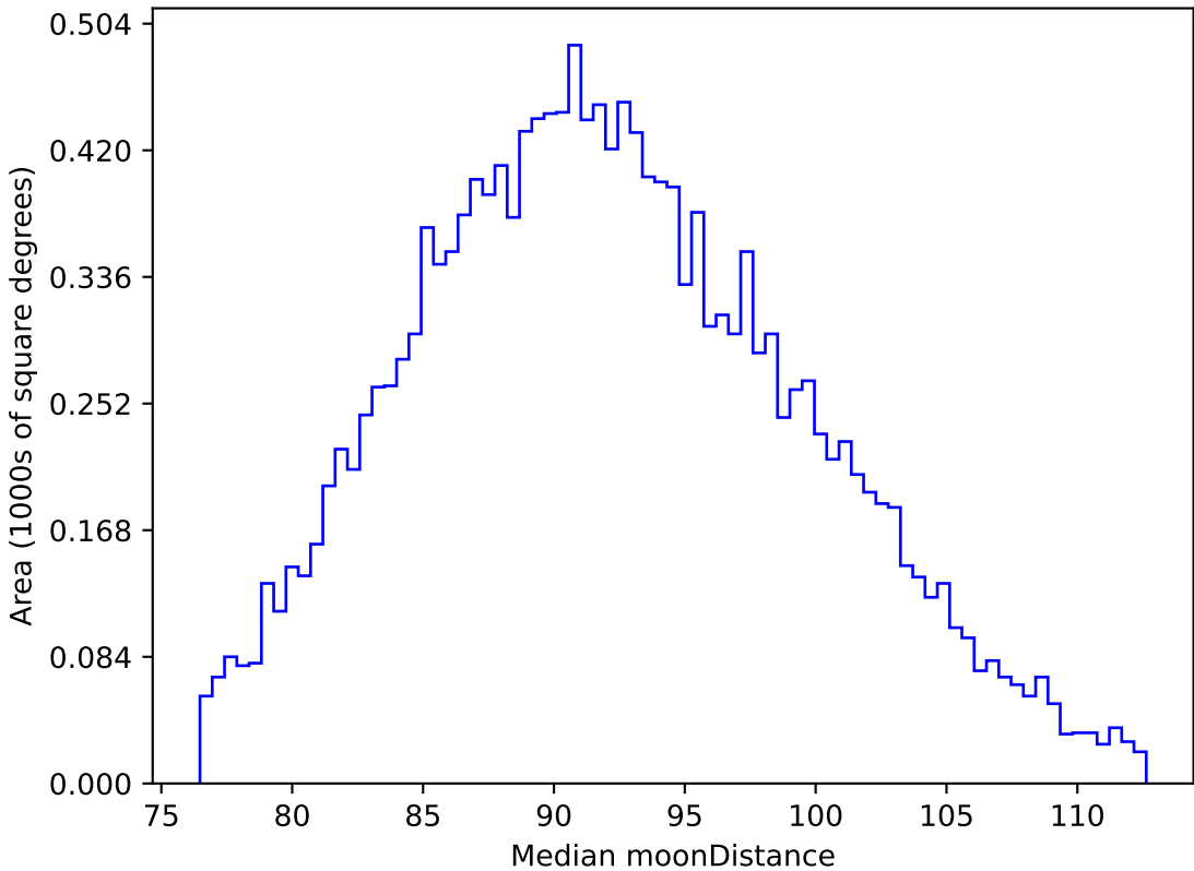
too_elab_r256_d3_griz_v3.4_10yrs WFD i band: Median moonDistance
