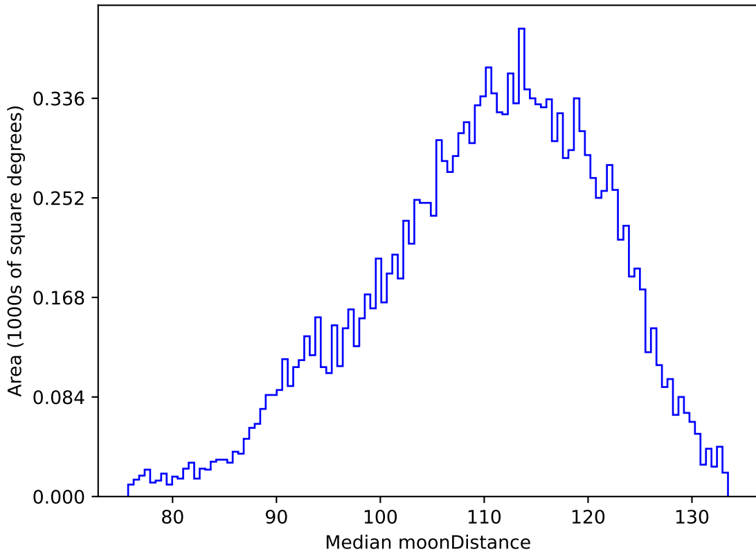
too_elab_r256_d3_griz_v3.4_10yrs WFD g band: Median moonDistance
