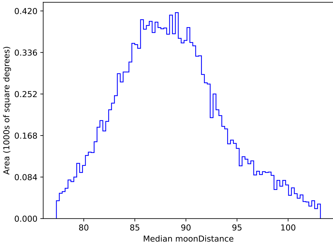
too_elab_r256_d3_griz_v3.4_10yrs WFD all bands: Median moonDistance
