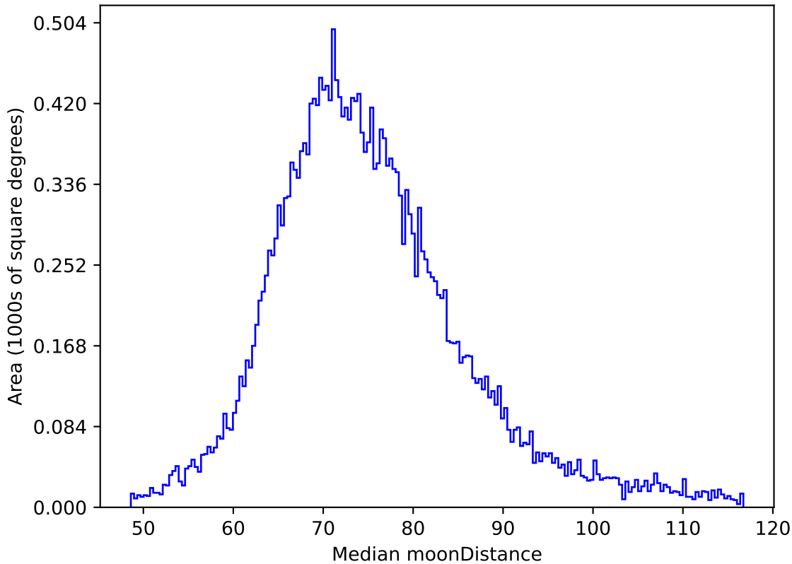
too_elab_r256_d3_griz_v3.4_10yrs All sky z band: Median moonDistance
