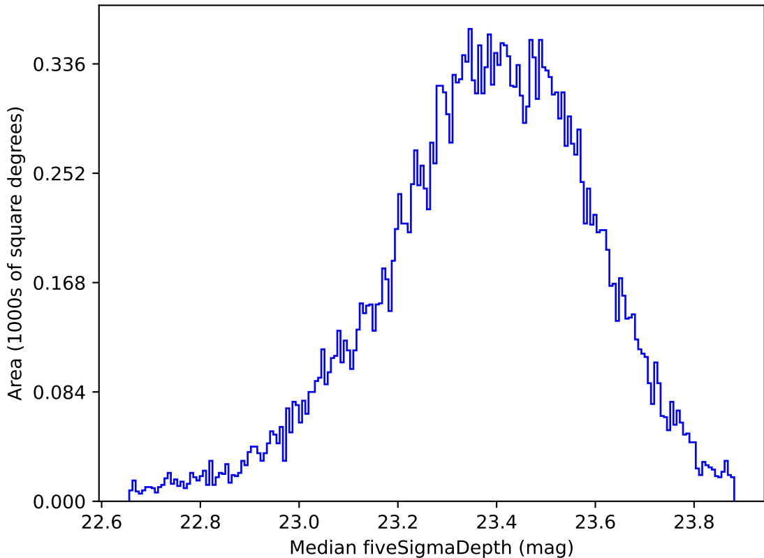
too_elab_r256_d3_griz_v3.4_10yrs Yr 1 all bands: Median fiveSigmaDepth
