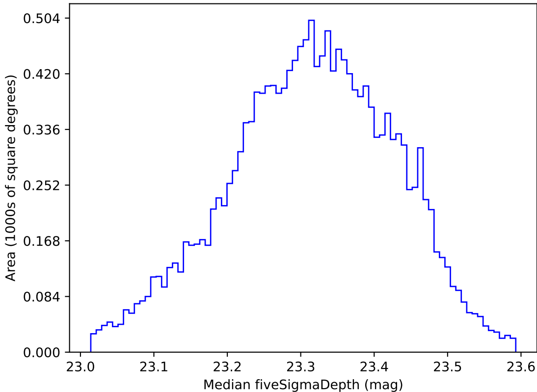
too_elab_r256_d3_griz_v3.4_10yrs WFD all bands: Median fiveSigmaDepth
