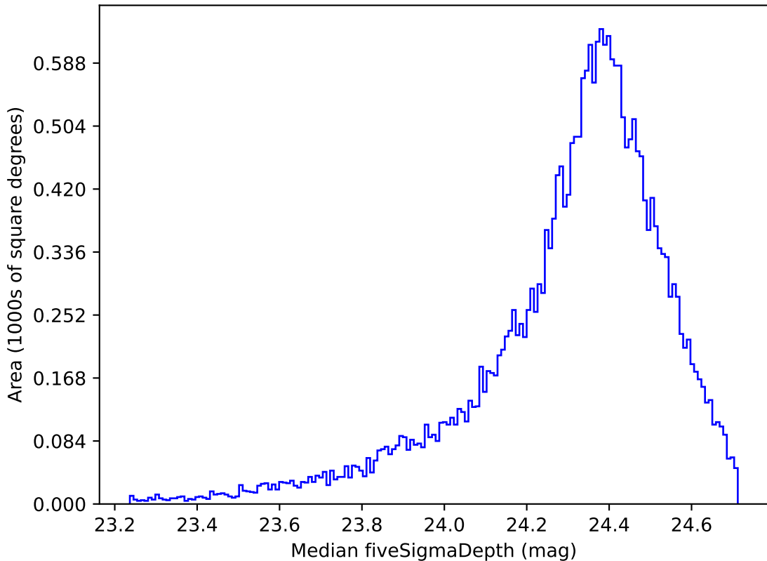
too_elab_r256_d3_griz_v3.4_10yrs All sky g band: Median fiveSigmaDepth
