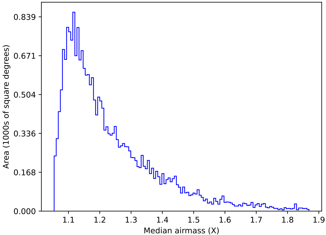
too_elab_r256_d3_griz_v3.4_10yrs Yr 1 u band: Median airmass
