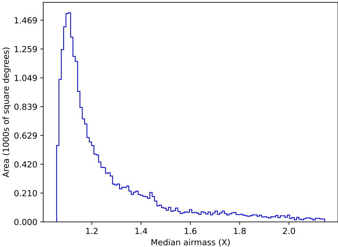
too_elab_r256_d3_griz_v3.4_10yrs Yr 1 r band: Median airmass
