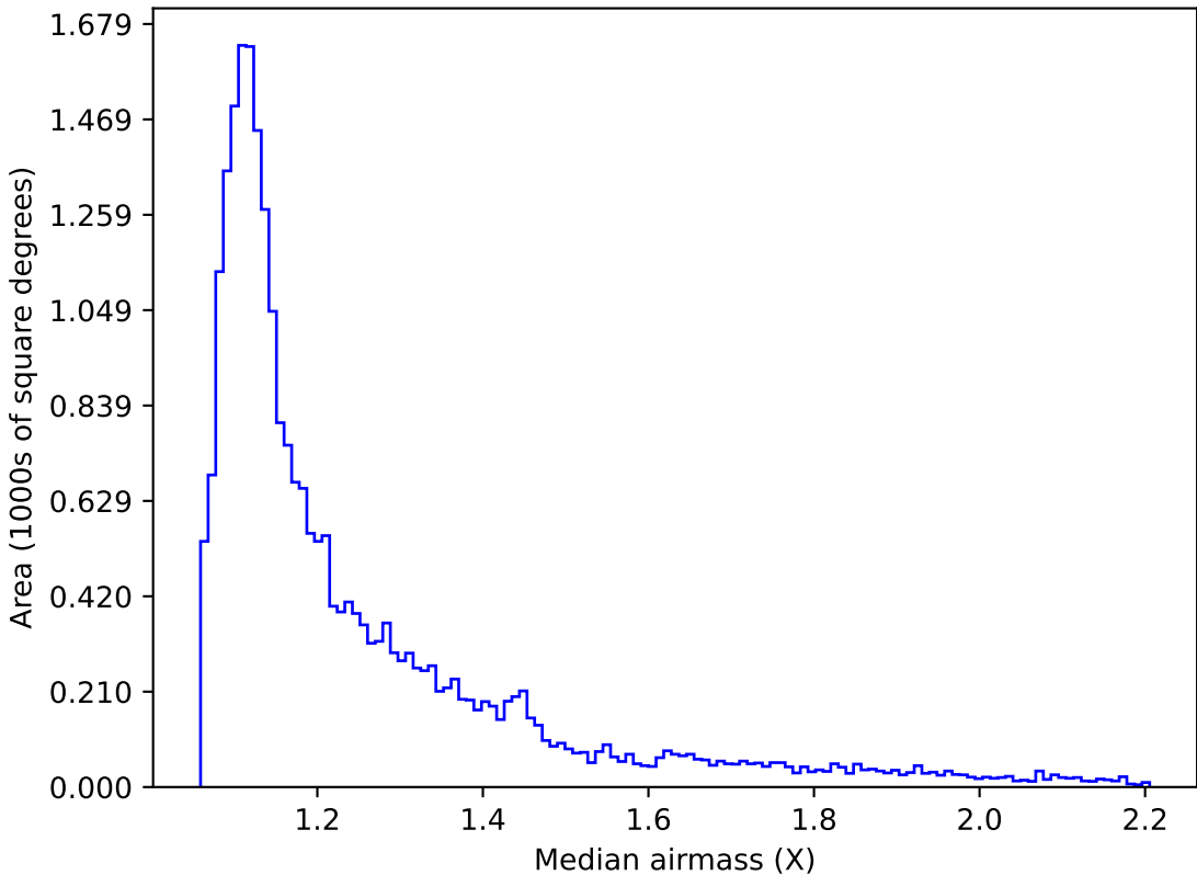
too_elab_r256_d3_griz_v3.4_10yrs Yr 1 i band: Median airmass
