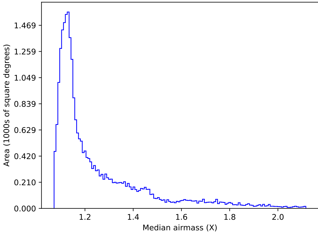
too_elab_r256_d3_griz_v3.4_10yrs Yr 1 all bands: Median airmass
