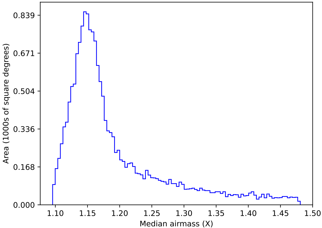
too_elab_r256_d3_griz_v3.4_10yrs WFD y band: Median airmass
