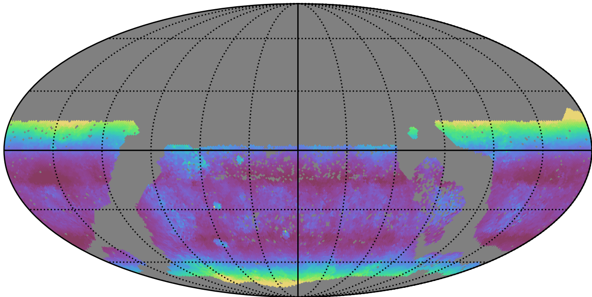
too_elab_r256_d3_griz_v3.4_10yrs WFD u band: Median airmass
