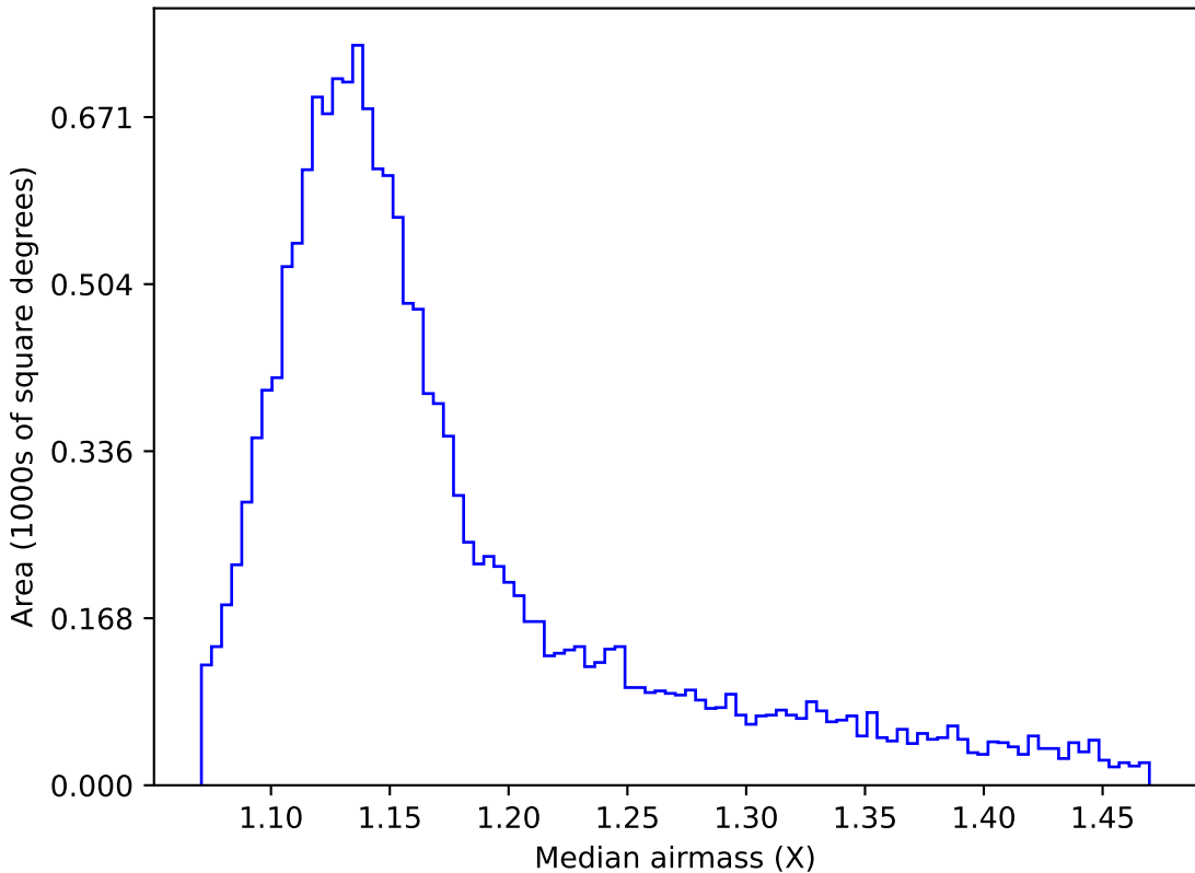
too_elab_r256_d3_griz_v3.4_10yrs WFD u band: Median airmass
