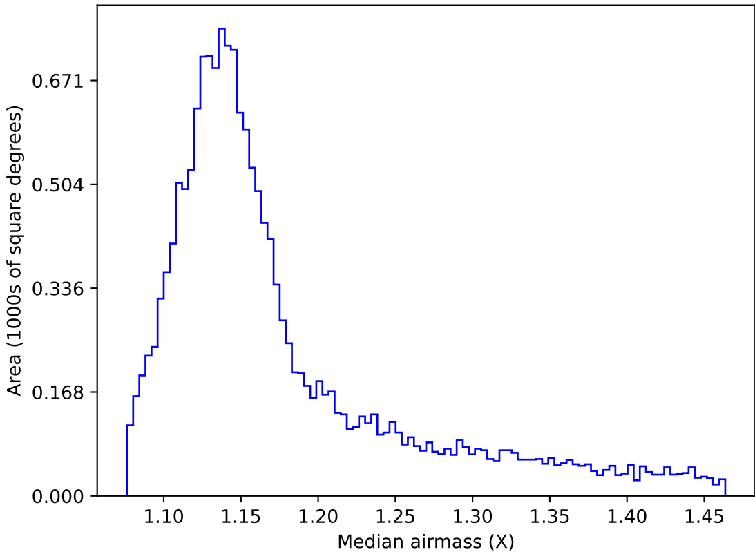
too_elab_r256_d3_griz_v3.4_10yrs WFD r band: Median airmass
