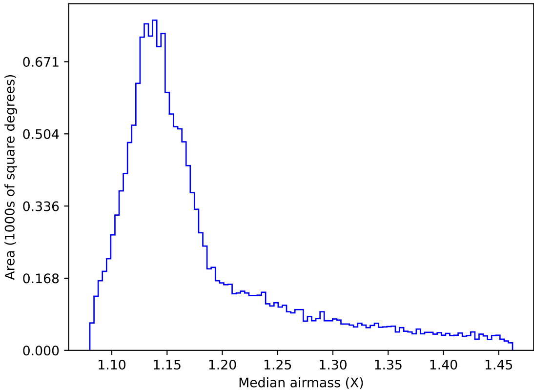
too_elab_r256_d3_griz_v3.4_10yrs WFD i band: Median airmass
