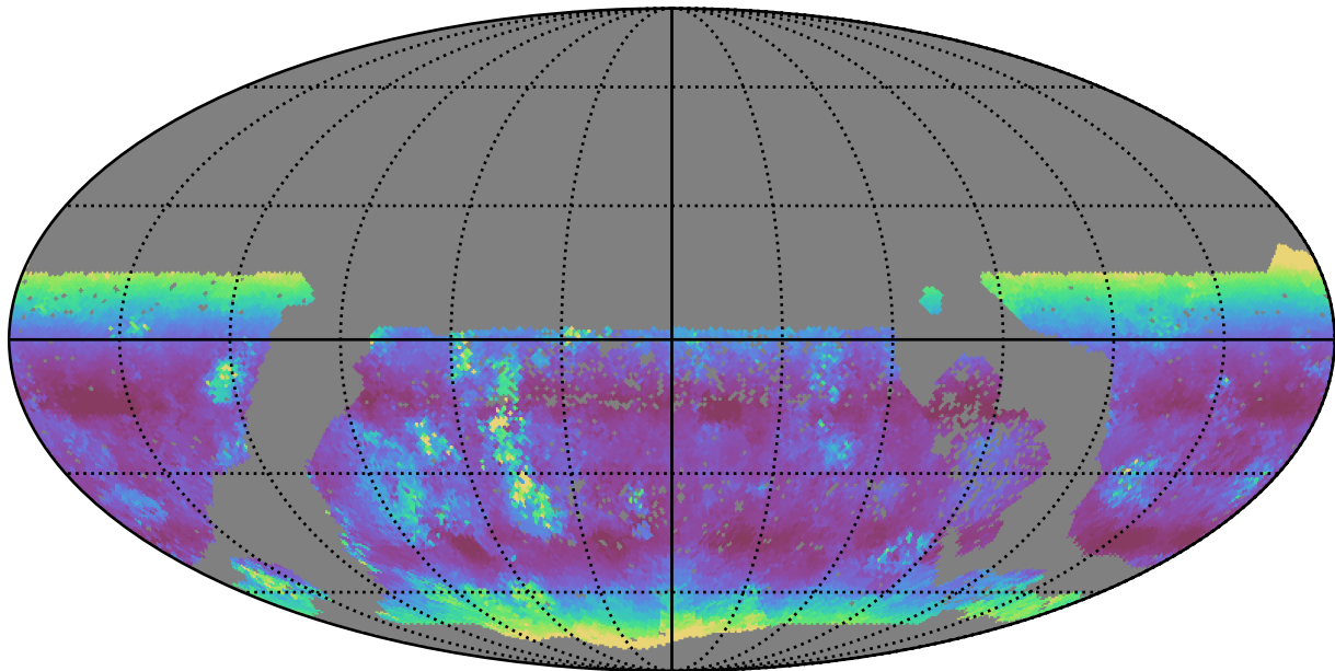
too_elab_r256_d3_griz_v3.4_10yrs WFD g band: Median airmass
