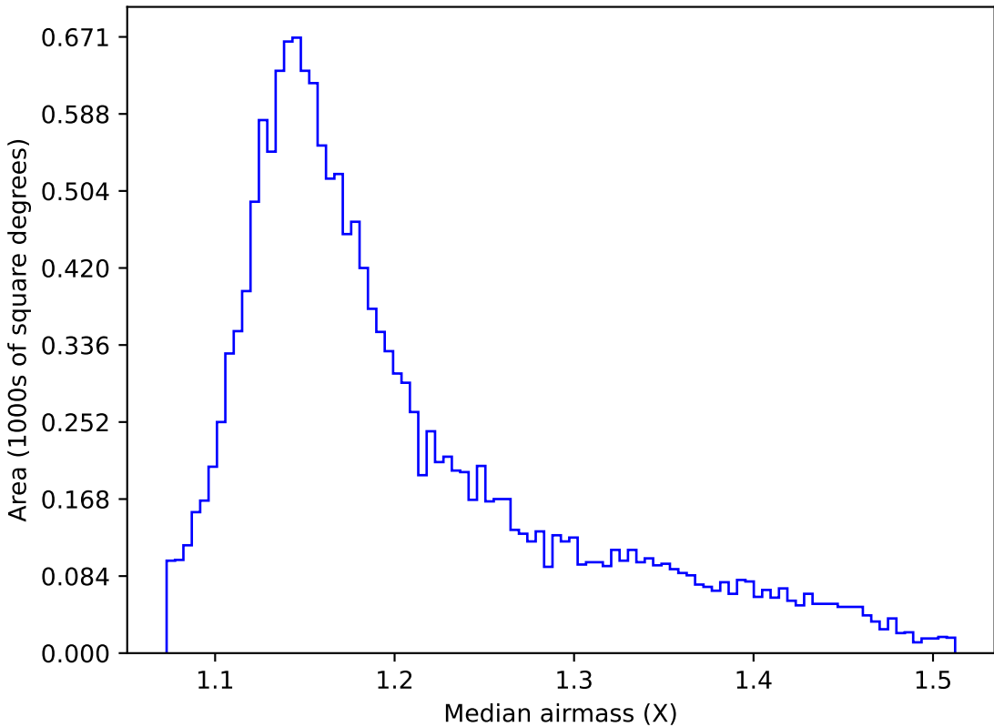
too_elab_r256_d3_griz_v3.4_10yrs WFD g band: Median airmass
