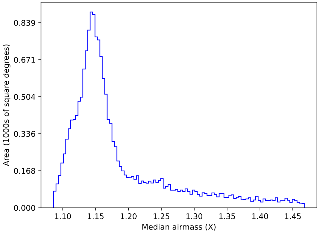
too_elab_r256_d3_griz_v3.4_10yrs WFD all bands: Median airmass
