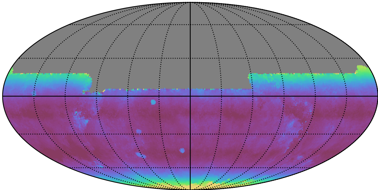
too_elab_r256_d3_griz_v3.4_10yrs All sky y band: Median airmass
