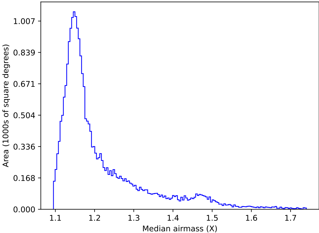
too_elab_r256_d3_griz_v3.4_10yrs All sky y band: Median airmass
