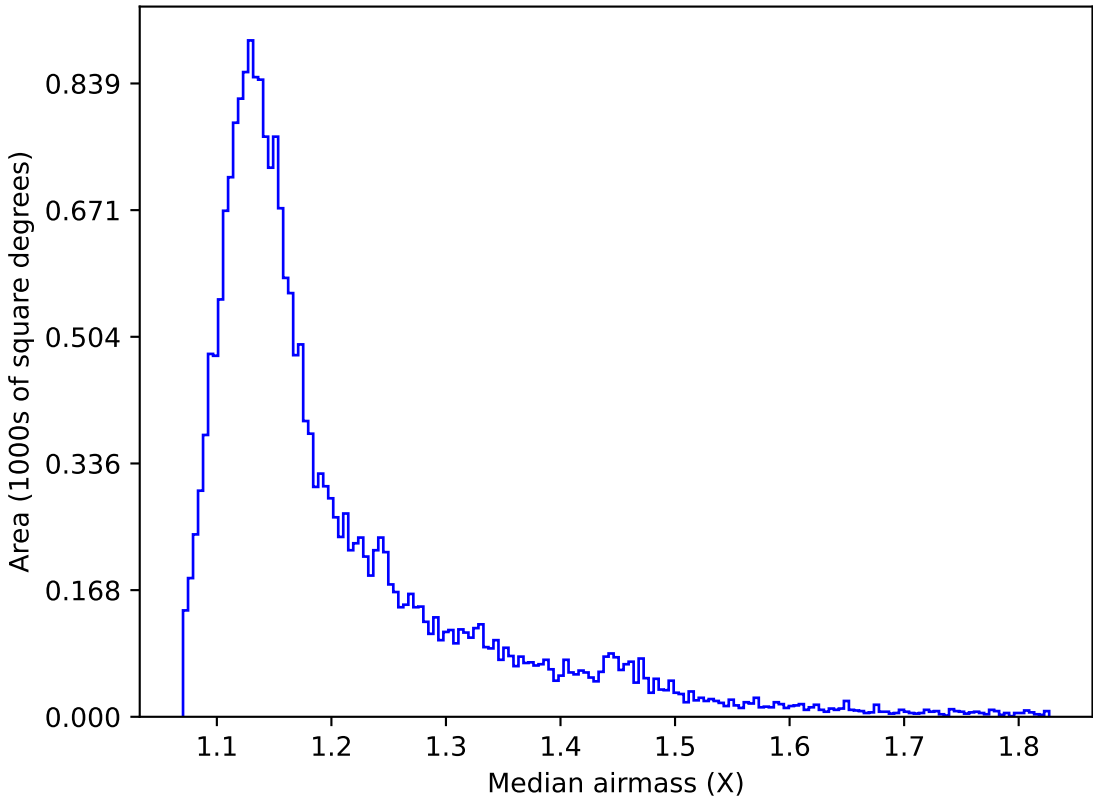
too_elab_r256_d3_griz_v3.4_10yrs All sky u band: Median airmass
