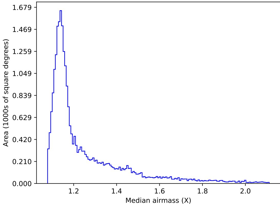
too_elab_r256_d3_griz_v3.4_10yrs All sky r band: Median airmass
