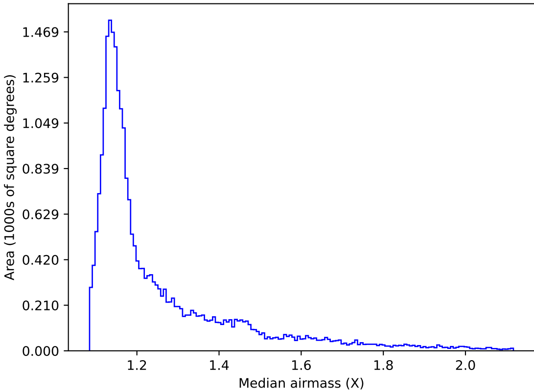
too_elab_r256_d3_griz_v3.4_10yrs All sky i band: Median airmass
