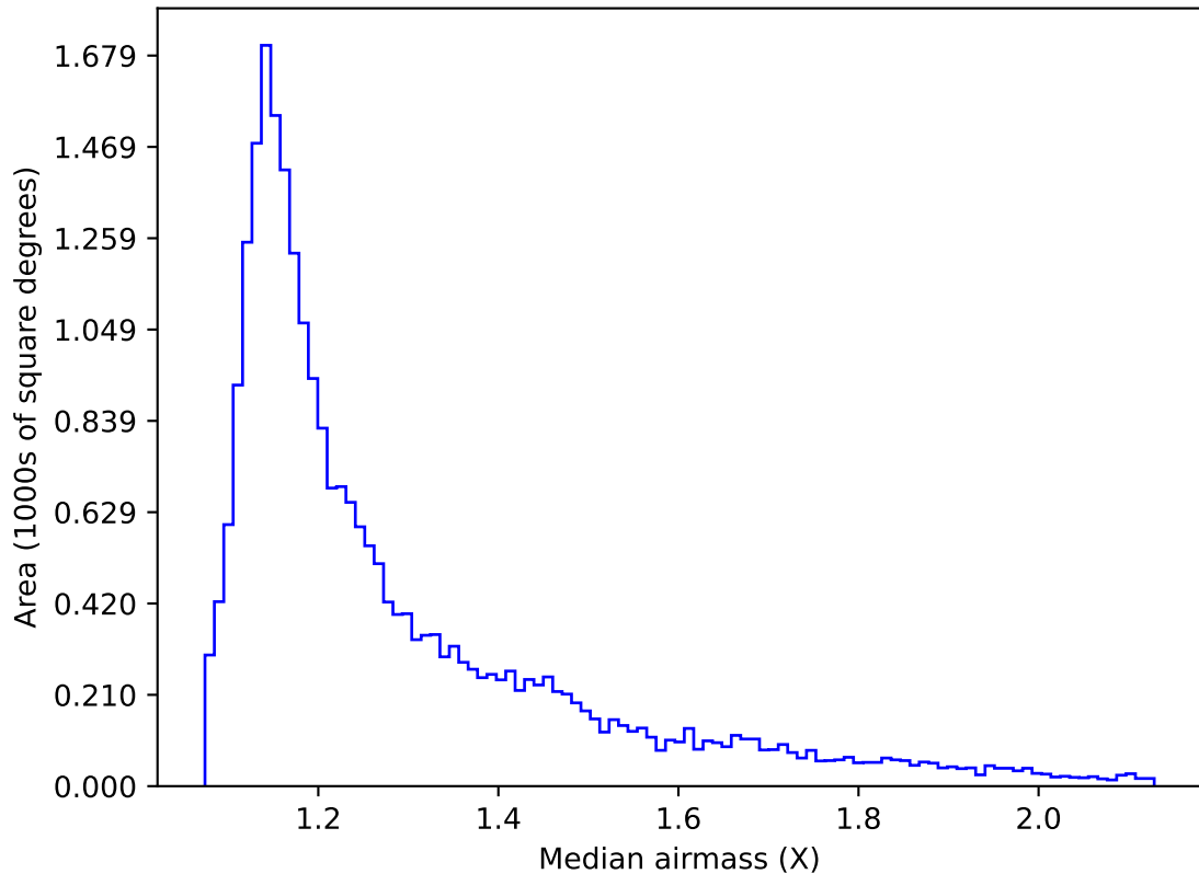
too_elab_r256_d3_griz_v3.4_10yrs All sky g band: Median airmass
