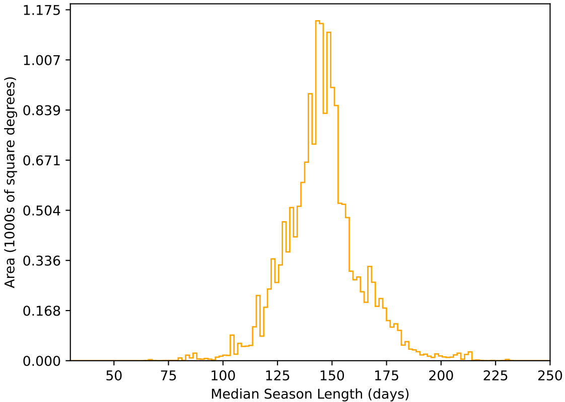
too_elab_r256_d3_griz_v3.4_10yrs WFD r band: Median Season Length
