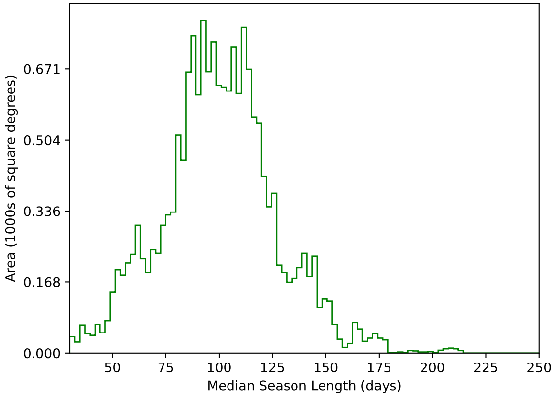
too_elab_r256_d3_griz_v3.4_10yrs WFD g band: Median Season Length
