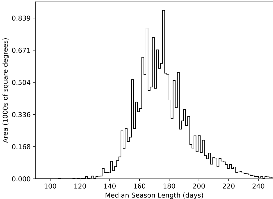
too_elab_r256_d3_griz_v3.4_10yrs WFD all bands: Median Season Length
