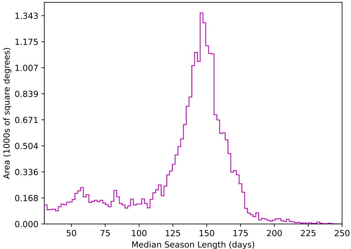
too_elab_r256_d3_griz_v3.4_10yrs All sky z band: Median Season Length
