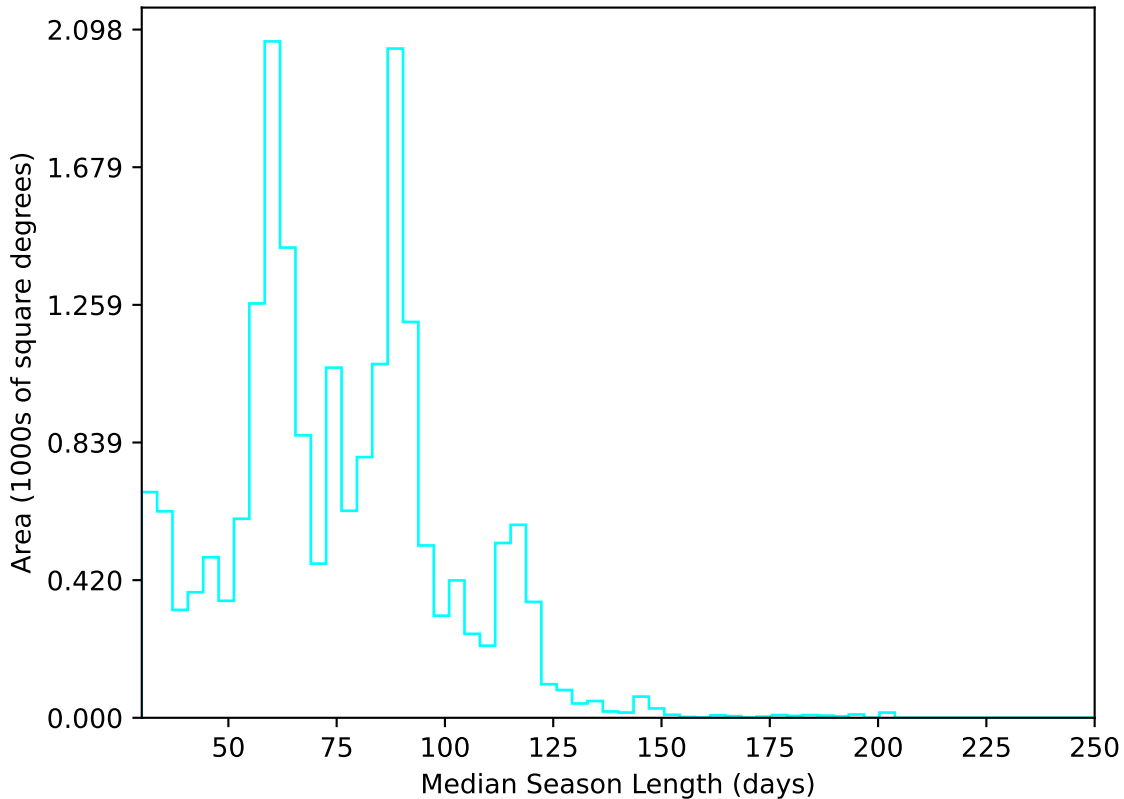
too_elab_r256_d3_griz_v3.4_10yrs All sky u band: Median Season Length
