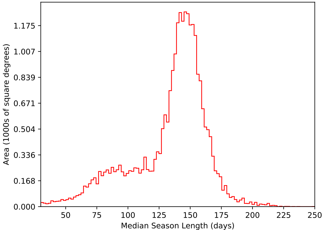
too_elab_r256_d3_griz_v3.4_10yrs All sky i band: Median Season Length
