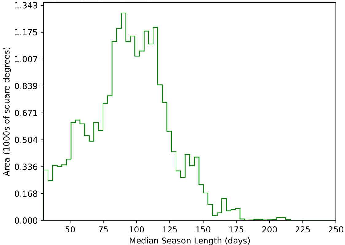
too_elab_r256_d3_griz_v3.4_10yrs All sky g band: Median Season Length
