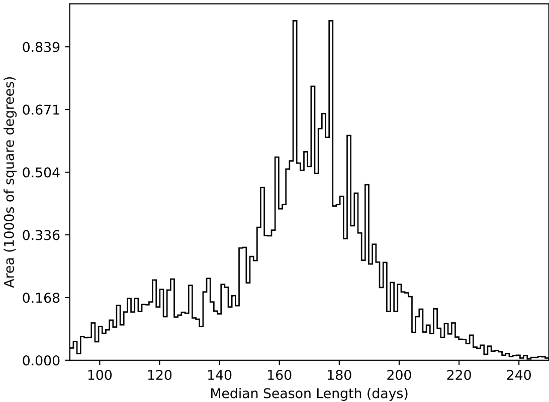
too_elab_r256_d3_griz_v3.4_10yrs All sky all bands: Median Season Length
