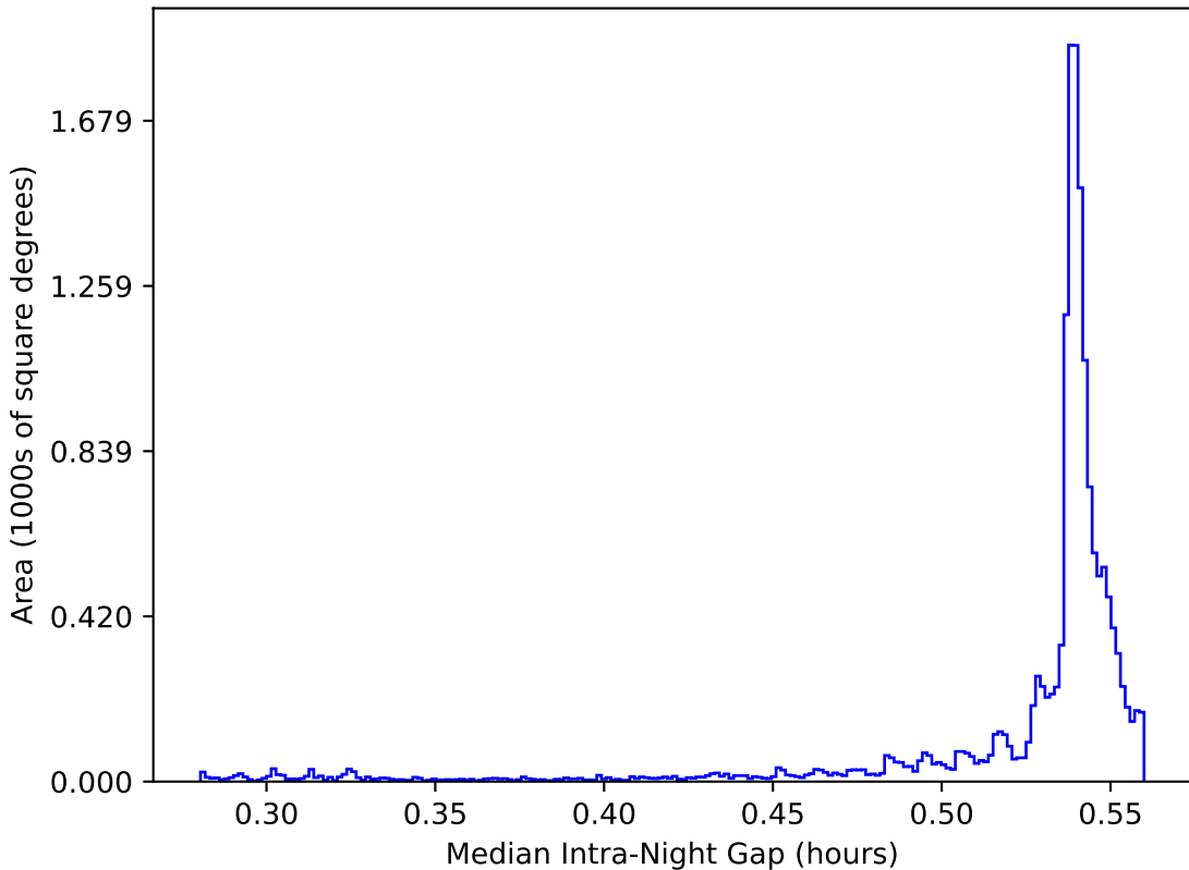
too_elab_r256_d3_griz_v3.4_10yrs WFD: Median Intra-Night Gap
