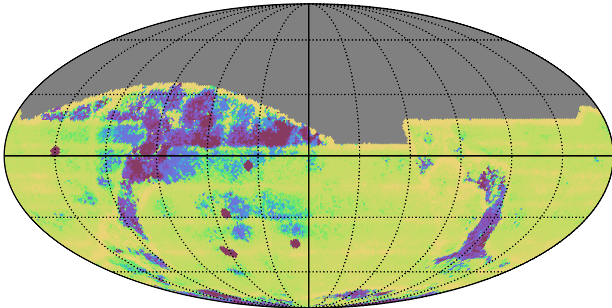
too_elab_r256_d3_griz_v3.4_10yrs All sky: Median Intra-Night Gap
