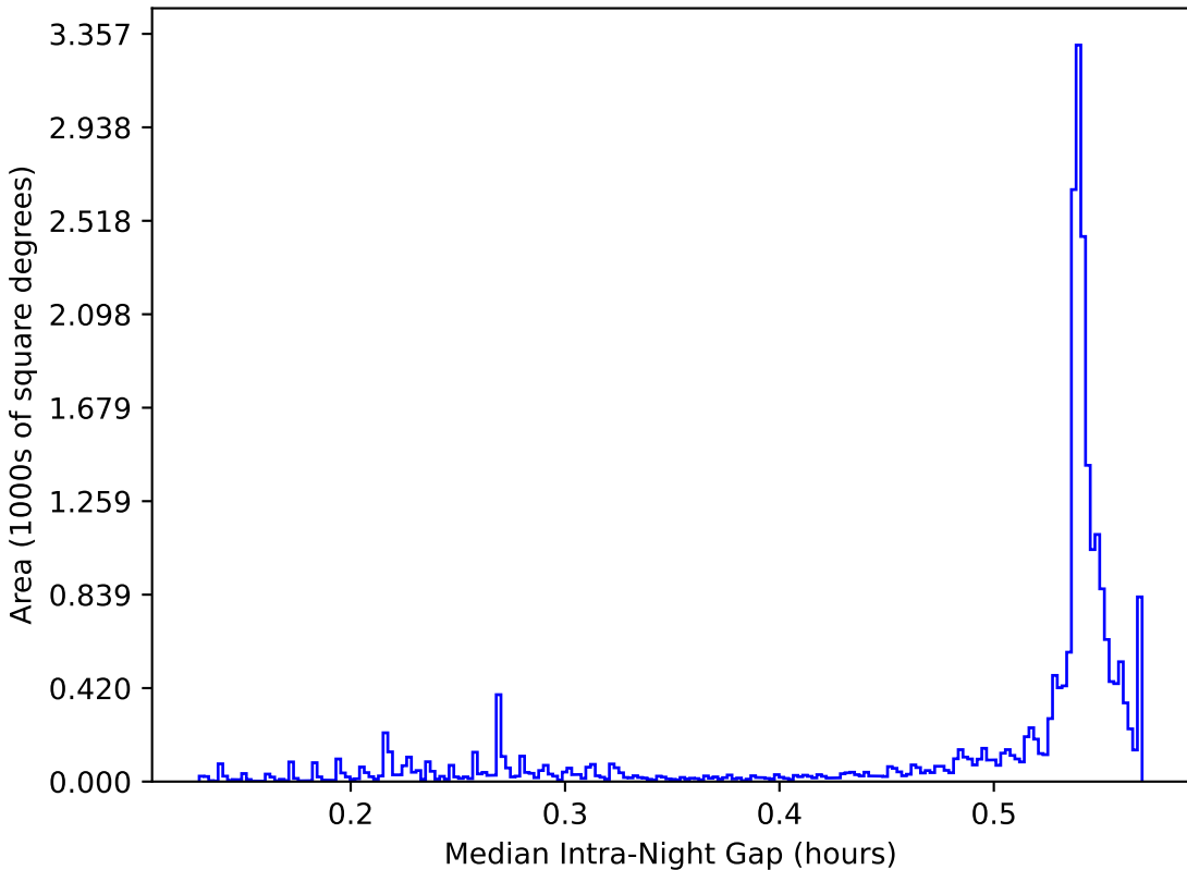
too_elab_r256_d3_griz_v3.4_10yrs All sky: Median Intra-Night Gap
