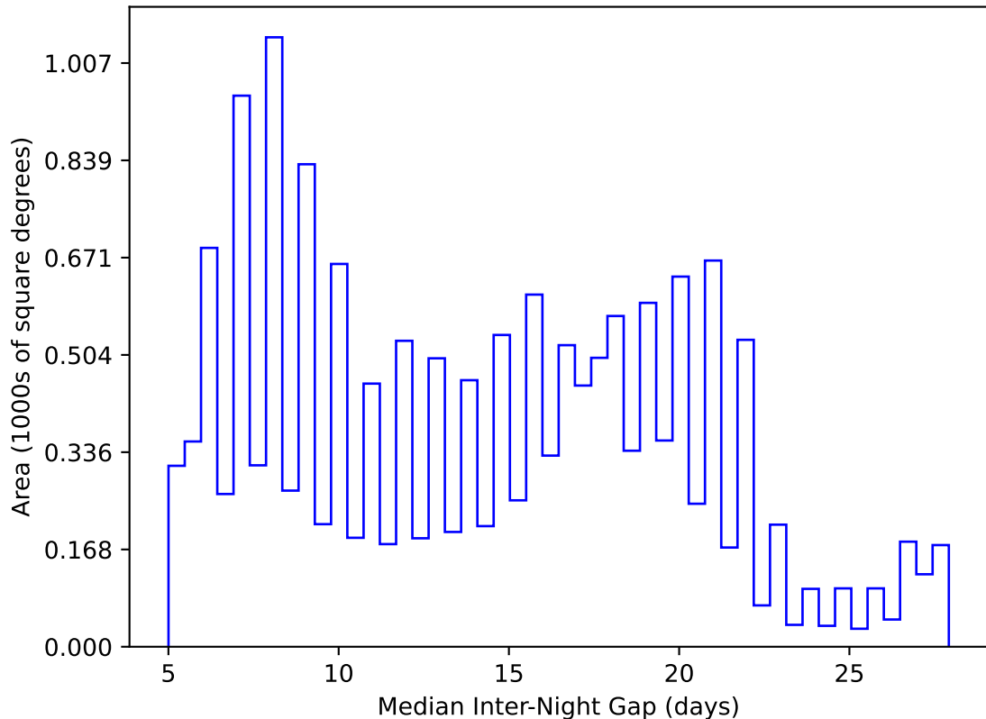
too_elab_r256_d3_griz_v3.4_10yrs WFD y band: Median Inter-Night Gap
