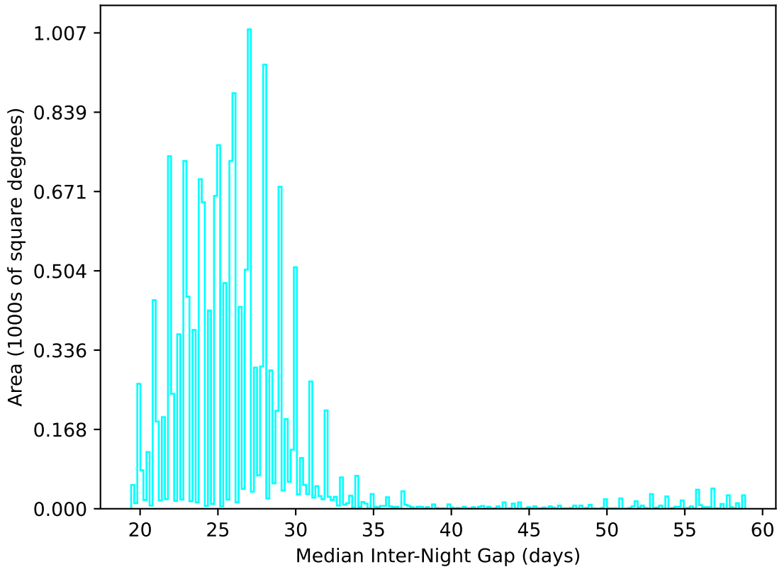
too_elab_r256_d3_griz_v3.4_10yrs WFD u band: Median Inter-Night Gap
