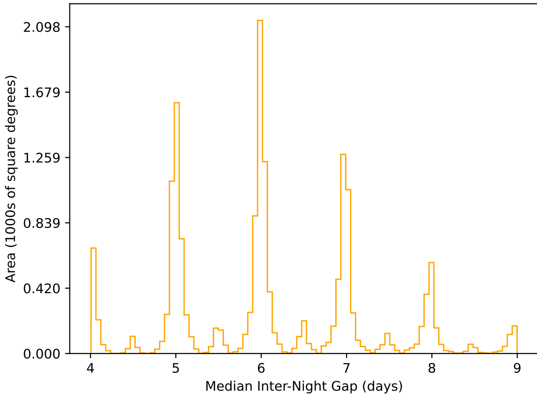
too_elab_r256_d3_griz_v3.4_10yrs WFD r band: Median Inter-Night Gap
