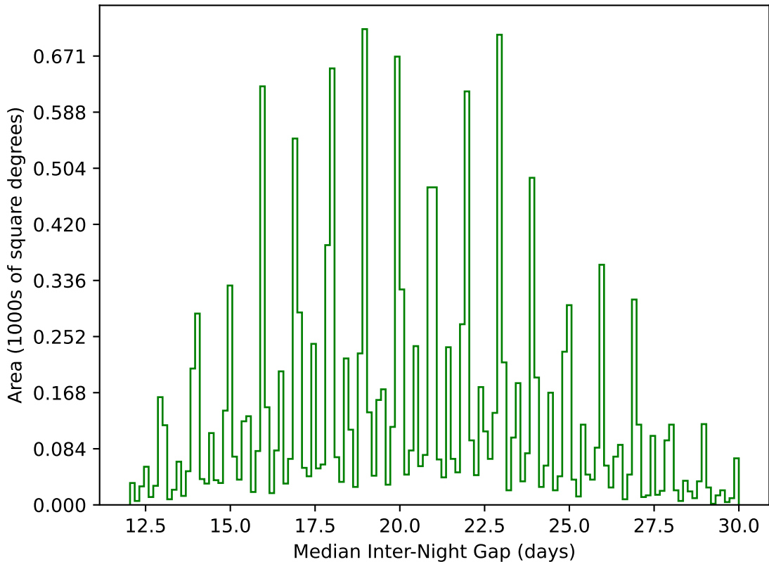
too_elab_r256_d3_griz_v3.4_10yrs WFD g band: Median Inter-Night Gap
