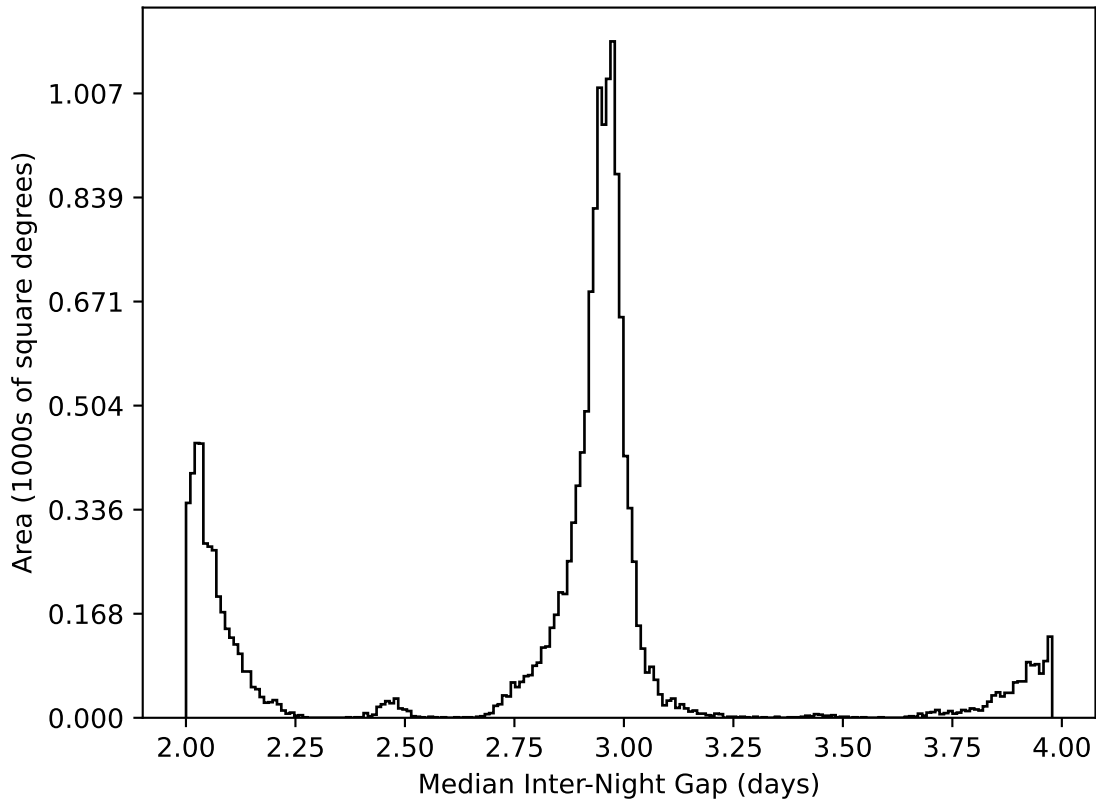
too_elab_r256_d3_griz_v3.4_10yrs WFD all bands: Median Inter-Night Gap
