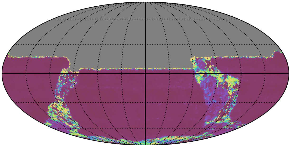
too_elab_r256_d3_griz_v3.4_10yrs All sky u band: Median Inter-Night Gap
