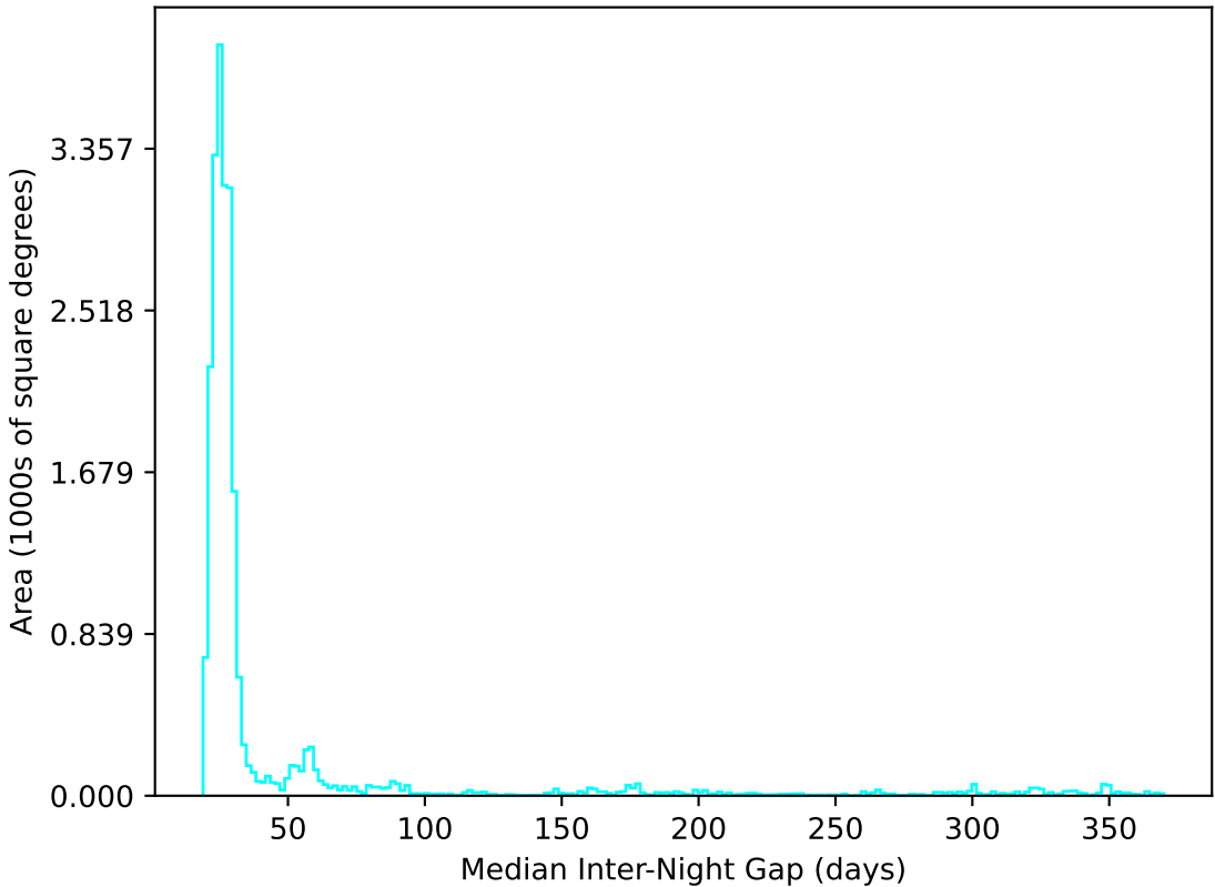
too_elab_r256_d3_griz_v3.4_10yrs All sky u band: Median Inter-Night Gap
