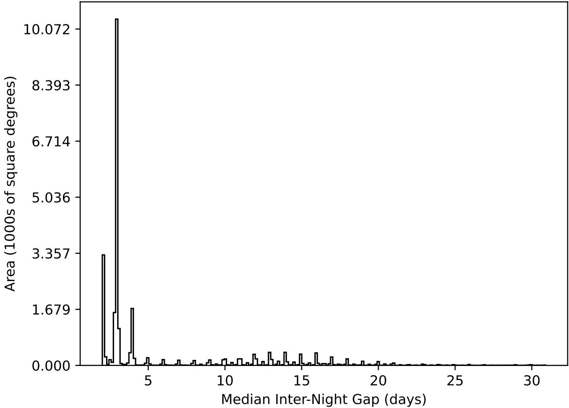
too_elab_r256_d3_griz_v3.4_10yrs All sky all bands: Median Inter-Night Gap
