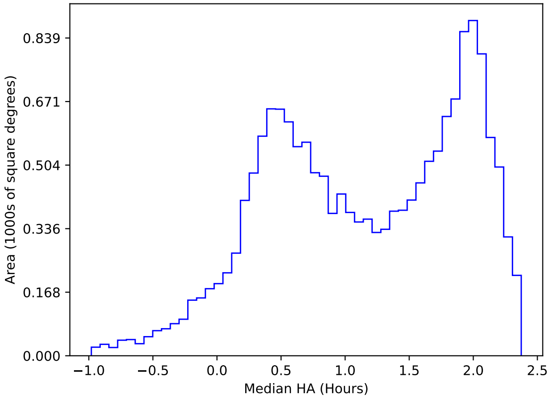
too_elab_r256_d3_griz_v3.4_10yrs WFD z band: Median HA
