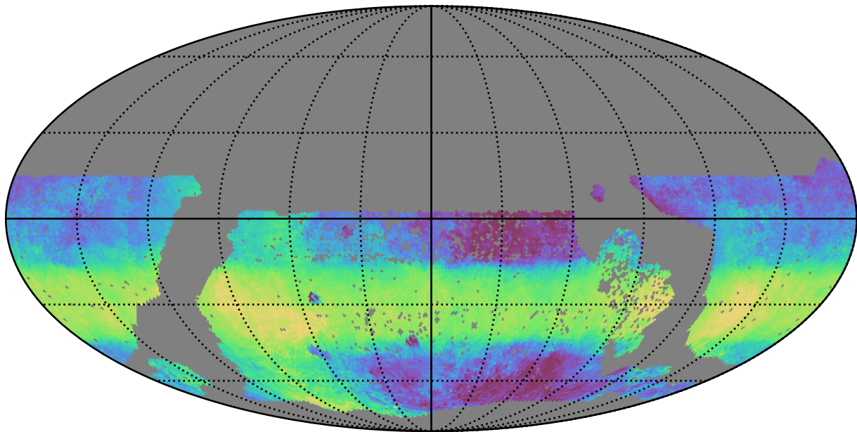
too_elab_r256_d3_griz_v3.4_10yrs WFD y band: Median HA
