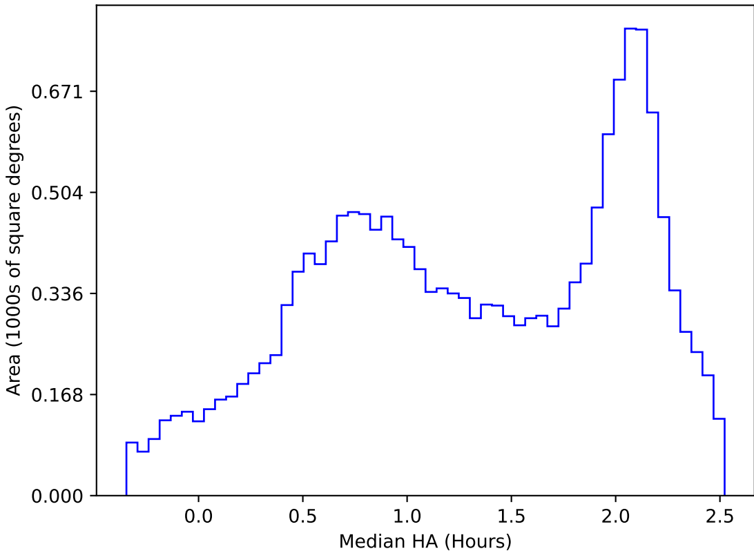
too_elab_r256_d3_griz_v3.4_10yrs WFD y band: Median HA
