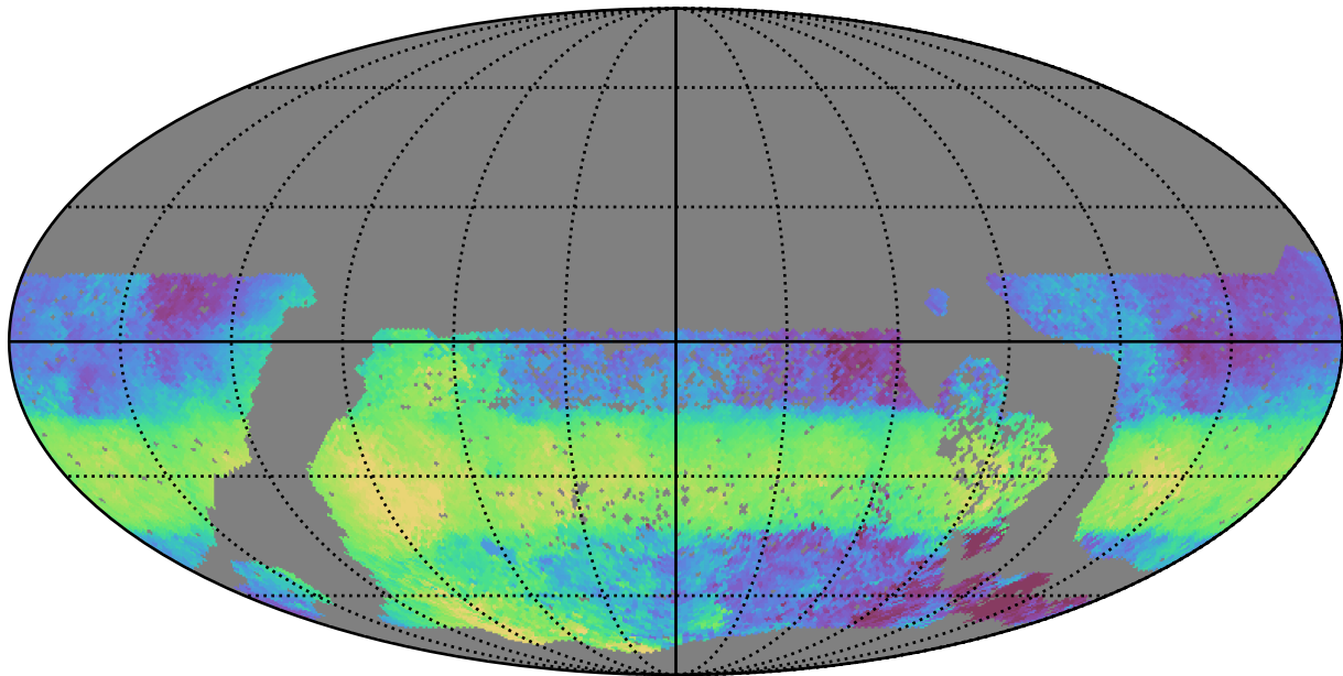
too_elab_r256_d3_griz_v3.4_10yrs WFD u band: Median HA
