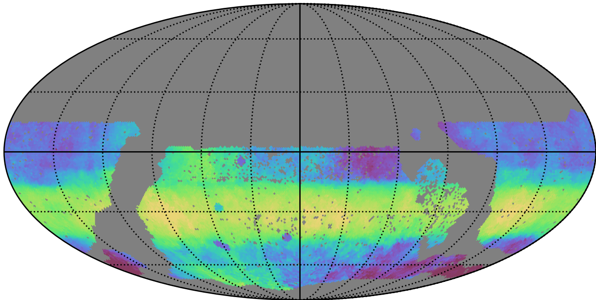
too_elab_r256_d3_griz_v3.4_10yrs WFD i band: Median HA
